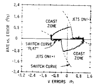
Fig. 13 Response to a ramp input, phase trajectory.
