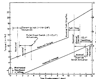
Fig. 2 Attitude controller assembly characteristics.
