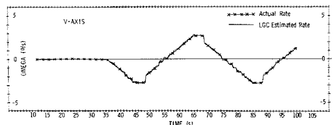
Fig. 12 Response to a ramp input, time history.
