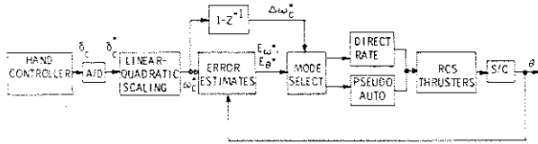
Fig. 5 Manual rate control logic.
